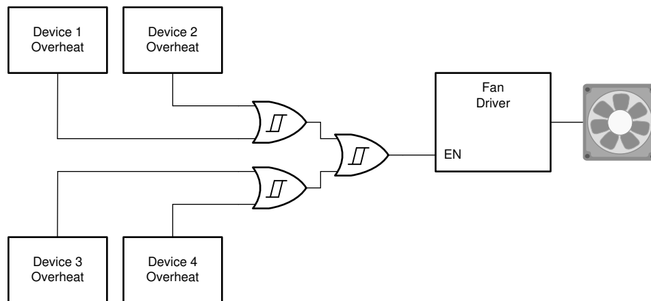
图 9. Typical application block diagram
