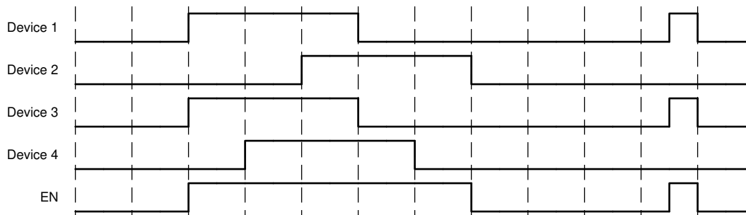
图 10. Application timing diagram
