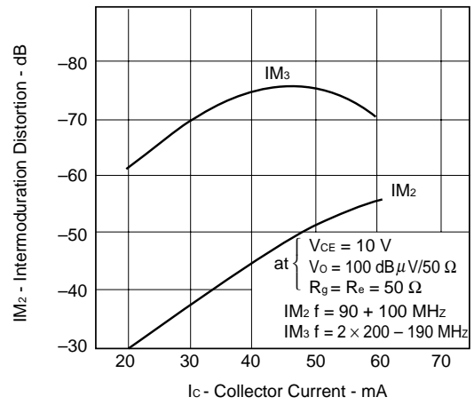
INTERMODULATION DISTORTION vs. COLLECTOR CURRENT
