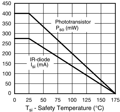
Fig. 1 - Derating Diagram
