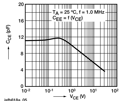
Fig. 7 - Transistor Capacitance
