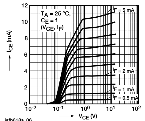
Fig. 8 - Output Characteristics
