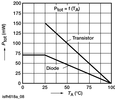
isfh618a_08 Fig. 10 - Permissible Power Dissipation
