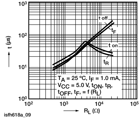
isfh618a_09 Fig. 11 - Switching Times (Typ.)
