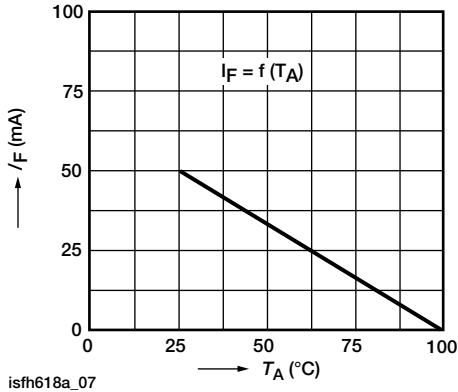
isfh618a_07 Fig. 9 - Permissible Forward Current Diode
