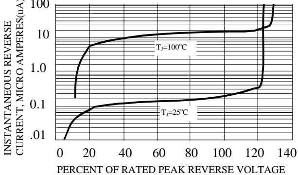
FIG. 4-TYPICAL REVERSE CHARACTERISTICS
