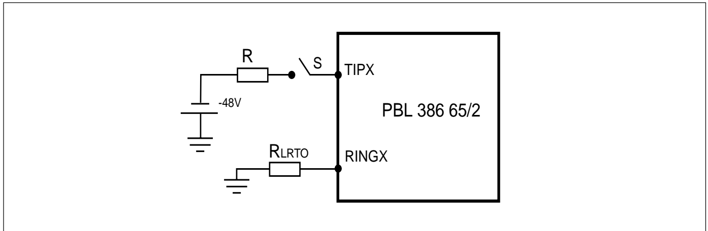
Figure 7. Tipx voltage.
