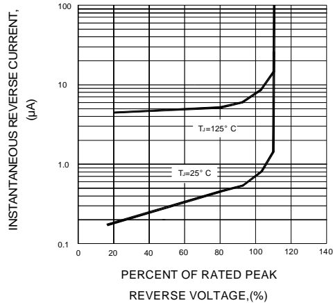
FIG.4-TYPICAL REVERSE CHARACTERISTICS
