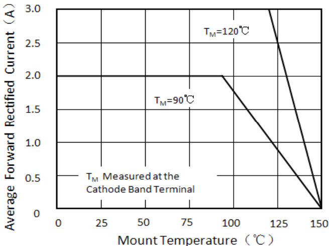
Figure 5. Forward Current Derating Curve
