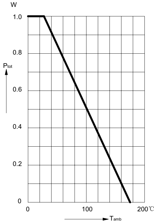
FIG.2 – ADMISSIBLE POWER DISSIPATION VERSUS AMBIENT TEMPERATURE
