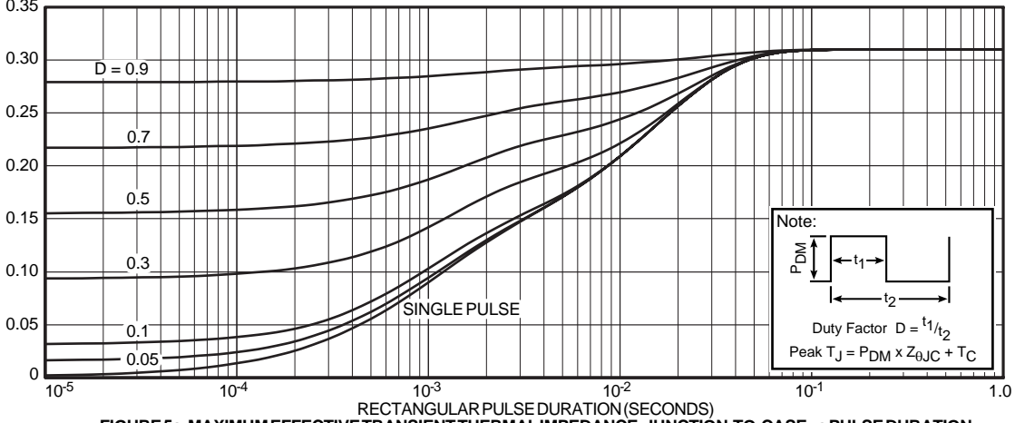
FIGURE 5a, MAXIMUM EFFECTIVE TRANSIENT THERMAL IMPEDANCE, JUNCTION-TO-CASE vs PULSE DURATION
