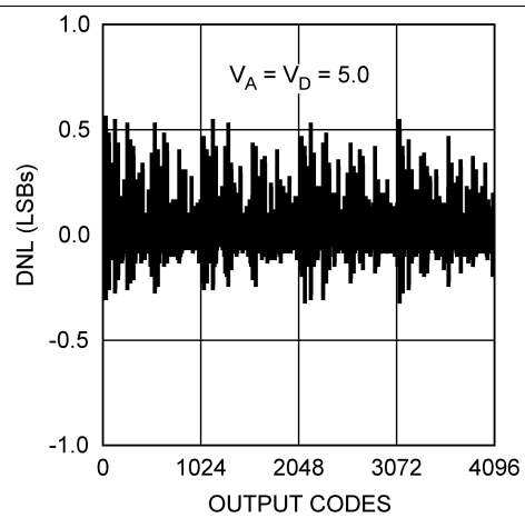
Figure 5. DNL
