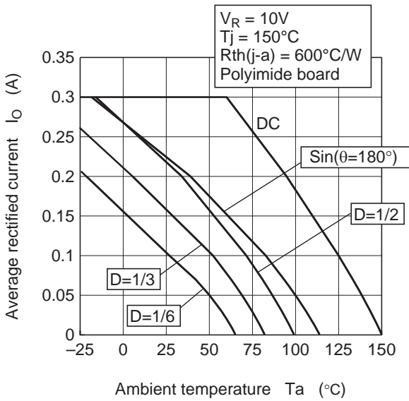
Fig.6 Average rectified current vs. Ambient temperature
