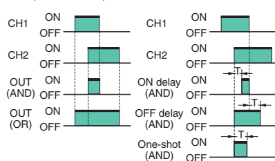
2. Control Output (AND, OR, Sync) and Timing Chart for Timer Settings (T: Set Time)
