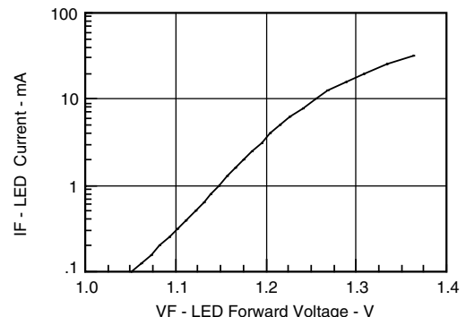
Fig. 4 - LED Forward Current vs. Forward Voltage
