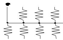
745X101 8 Resistors 10 Terminations
