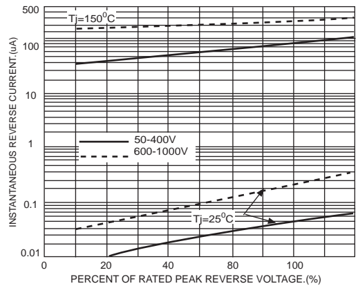
FIG.4-TYPICAL REVERSE CHARACTERISTICS PER BRIDGE ELEMENT (GBU6005 THRU GBU810)
