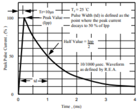
Fig. 5 - Pulse Waveform
