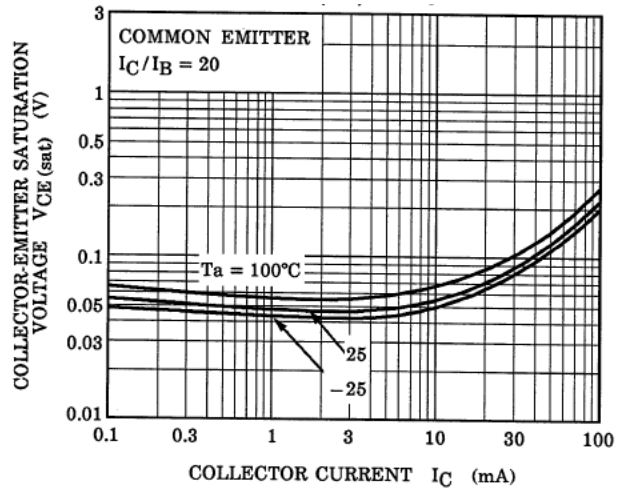
Fig. 9.8 RN1911FE V_{CE(sat)}-I_C
