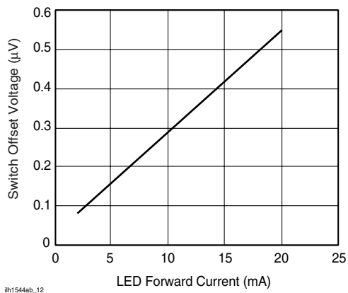
Figure 13. Switch Offset Voltage vs. LED Current
