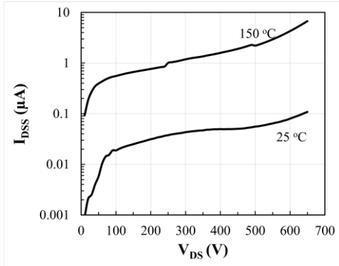
Typical off-state drain leakage current I_{DSS} vs. V_{DS} @ T_J = 25\text{ }^\circ\text{C} and 150\text{ }^\circ\text{C}
