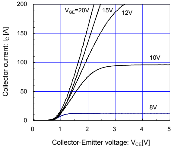
[ Inverter ] Collector current vs. Collector-Emmitter voltage (typ.) Tj= 25°C / chip
