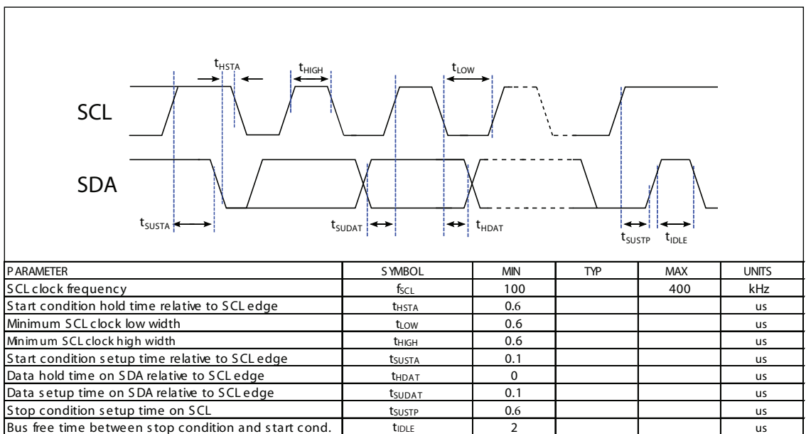
Figure 6 - I2C Timing Diagram
