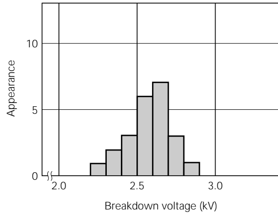
(a) Between Coil and Contacts (n = 25 pcs)
