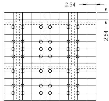
Mounting Layout (mm)
