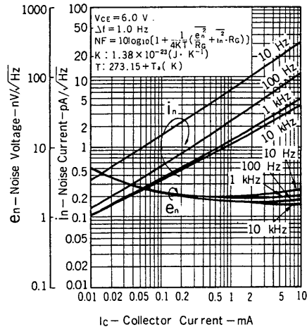
e_n AND i_n vs. COLLECTOR CURRENT
