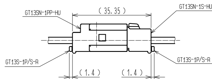
MATED CONNECTORS
