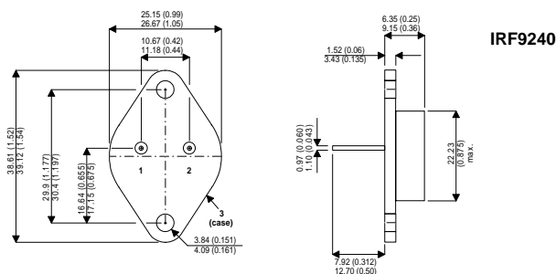
TO-3 Package (TO-204AA)
