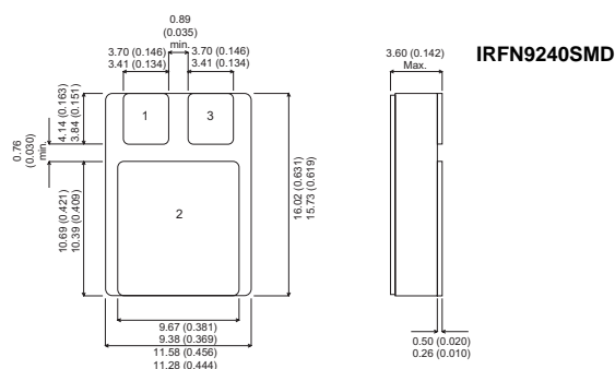
SMD1 (TO276AB)
