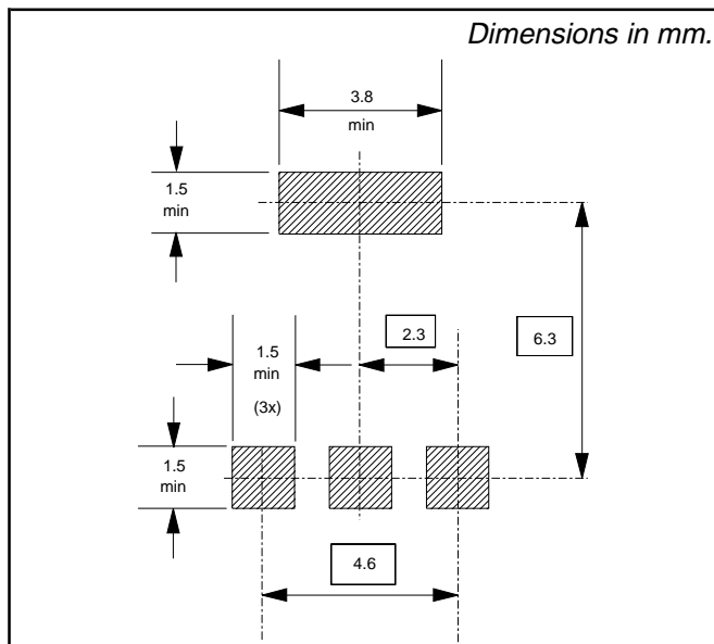
Fig.18. Soldering pattern for surface mounting.
