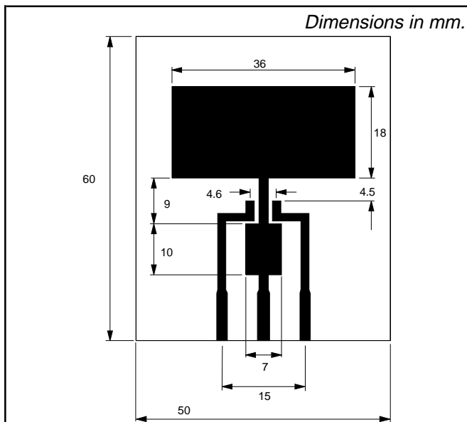
Fig.19. PCB for thermal resistance and power rating. PCB: FR4 epoxy glass (1.6 mm thick), copper laminate (35 μm thick).
