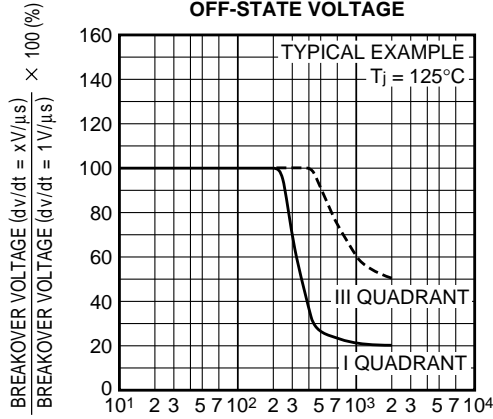
RATE OF RISE OF OFF-STATE VOLTAGE ( V/\mu s )
