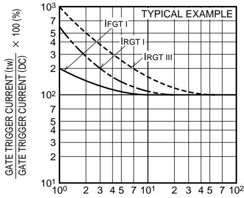
GATE CURRENT PULSE WIDTH ( \mu s )
