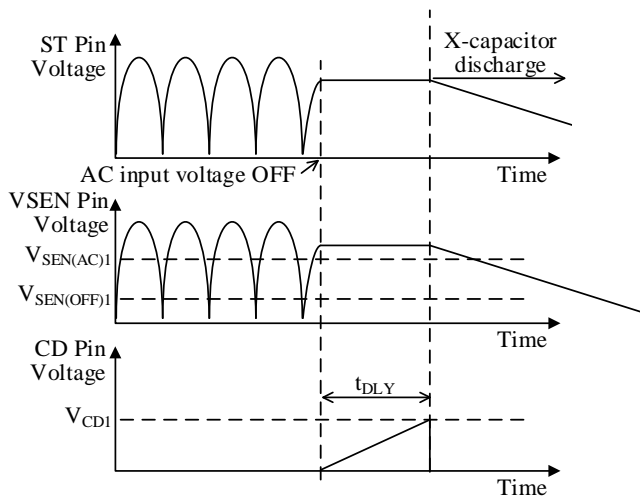
Figure 8-32. Operational Waveform of X-capacitor Discharge Function
