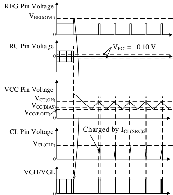
Figure 8-35. REG_OVP Waveform
