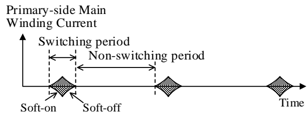
Figure 8-19. Standby Waveform
