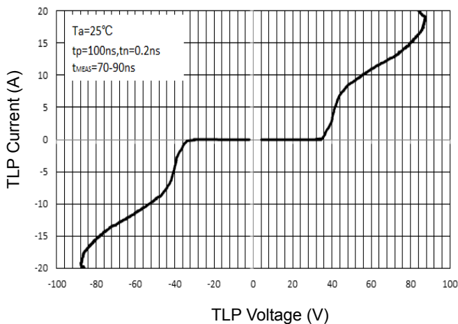
Fig 5. TLP Curve
