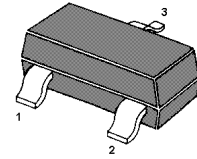
Marking Code: EA1 SOT-23 Plastic Package
