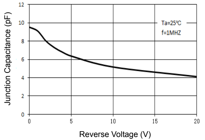
Fig 4. Junction Capacitance
