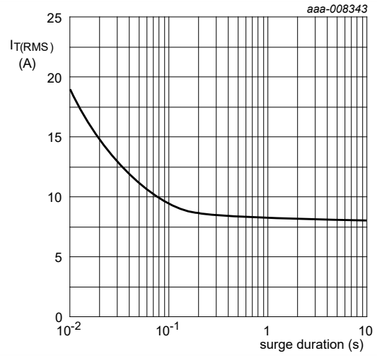
Fig. 3. RMS on-state current as a function of surge duration; maximum values f = 50 \text{ Hz}; T_{mb} = 135 \text{ °C}
