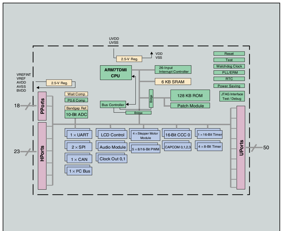
Fig. 2: Block diagram of the CDC 3231G
