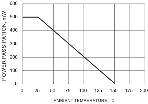
FIG. 1-POWER DISSIPATION VS. AMBIENT TEMP.
