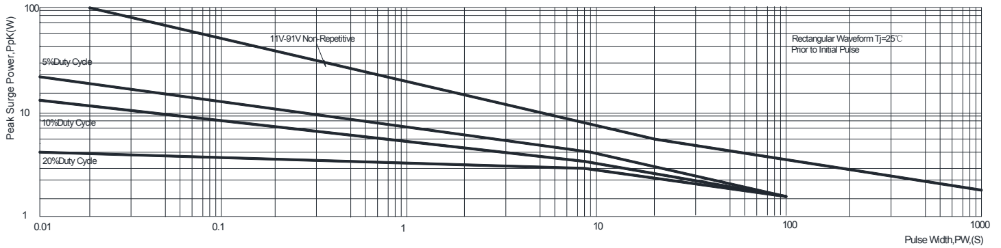
FIG5: Maximum Surge Power
