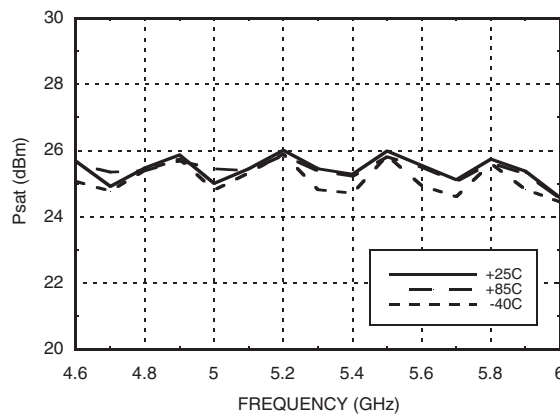
Bypass Mode P sat vs. Temperature [1]
