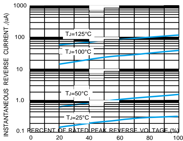
FIG.5-TYPICAL REVERSE CHARACTERISTICS
