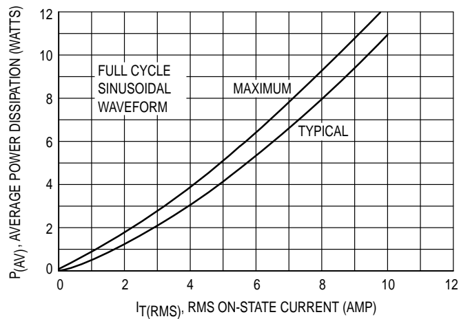
FIGURE 2 – POWER DISSIPATION
