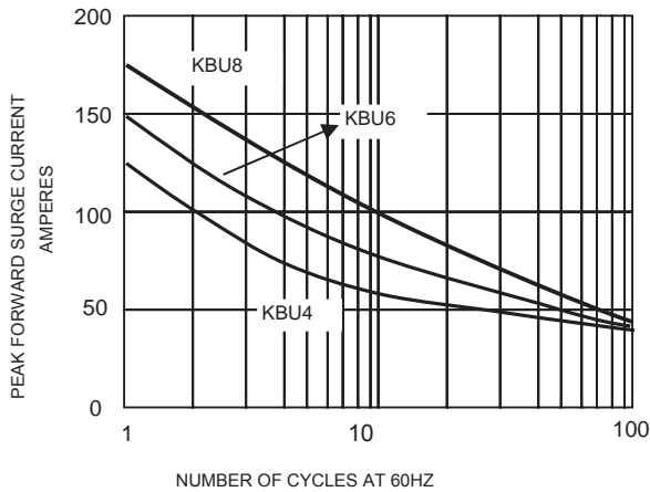
FIG.3-MAXIMUM NON-RETTITIVE PEAK FORWARD SURGE CURRENT
