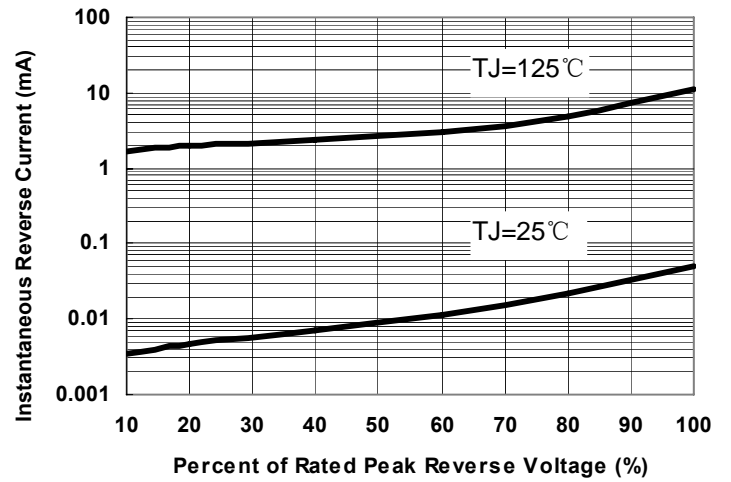
Fig.2-Typical Reverse Characteristics
