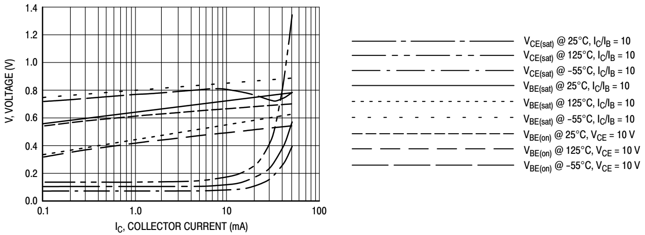
Figure 3. "ON" Voltages
