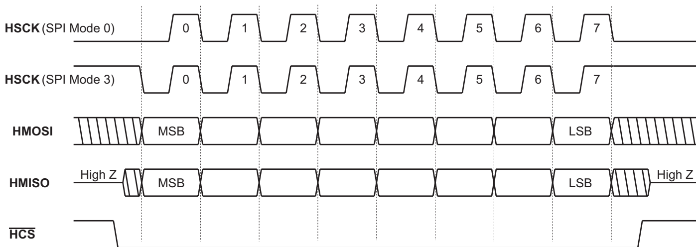
FIGURE 2. Generalized Single-Byte Transfer Using SPI Protocol, HSClock is Shown for SPI Modes 0 and 3
