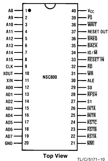
Dual-In-Line Package
