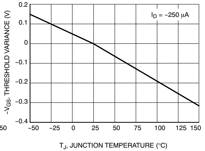
Figure 8. Threshold Voltage
