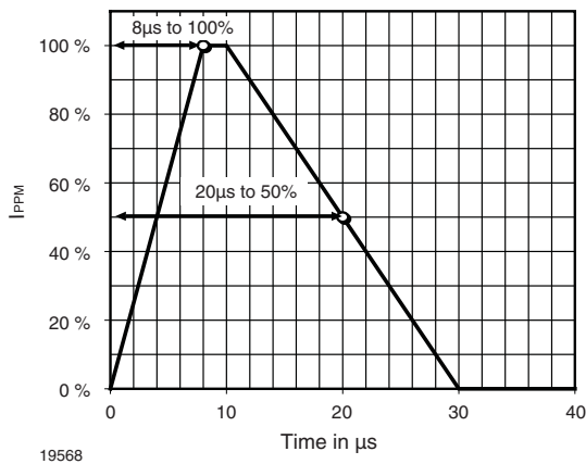
Figure 1. 8/20µs Peak Pulse Current wave form acc. IEC 61000-4-5
