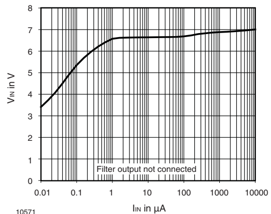
Figure 4. Typical Input Voltage V_{IN} vs. Input Current I_{IN}
