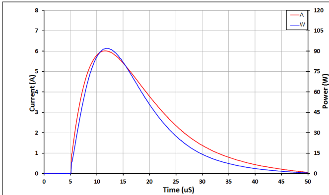
图 6-7. Negative Surge Waveform 8 to 20 µs
