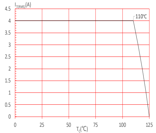
FIG.4: On-state characteristics
