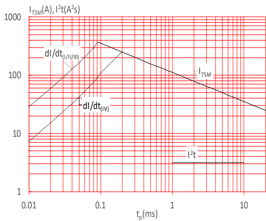
FIG.5: Non-repetitive surge peak on-state current for a sinusoidal pulse with width t_p < 20\text{ms} , and corresponding value of I^2t ( I - II -III: di/dt < 30\text{A}/\mu\text{s} ; IV: di/dt < 20\text{A}/\mu\text{s} )
