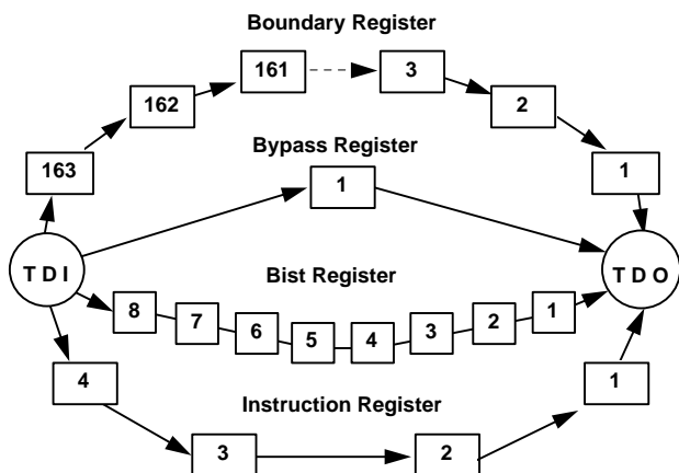
Figure 10. JTAG Registers
