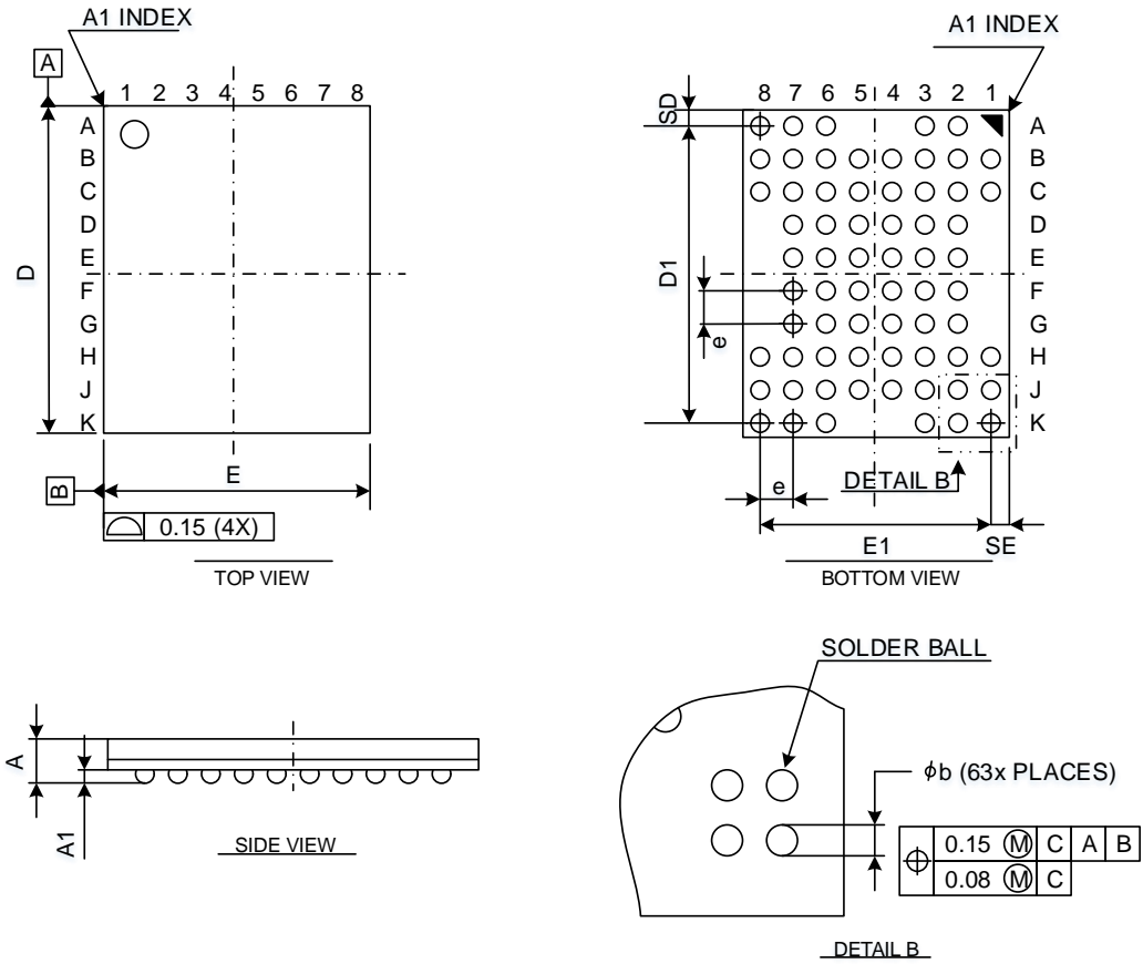
Figure 13-3: FBGA-67 figures
