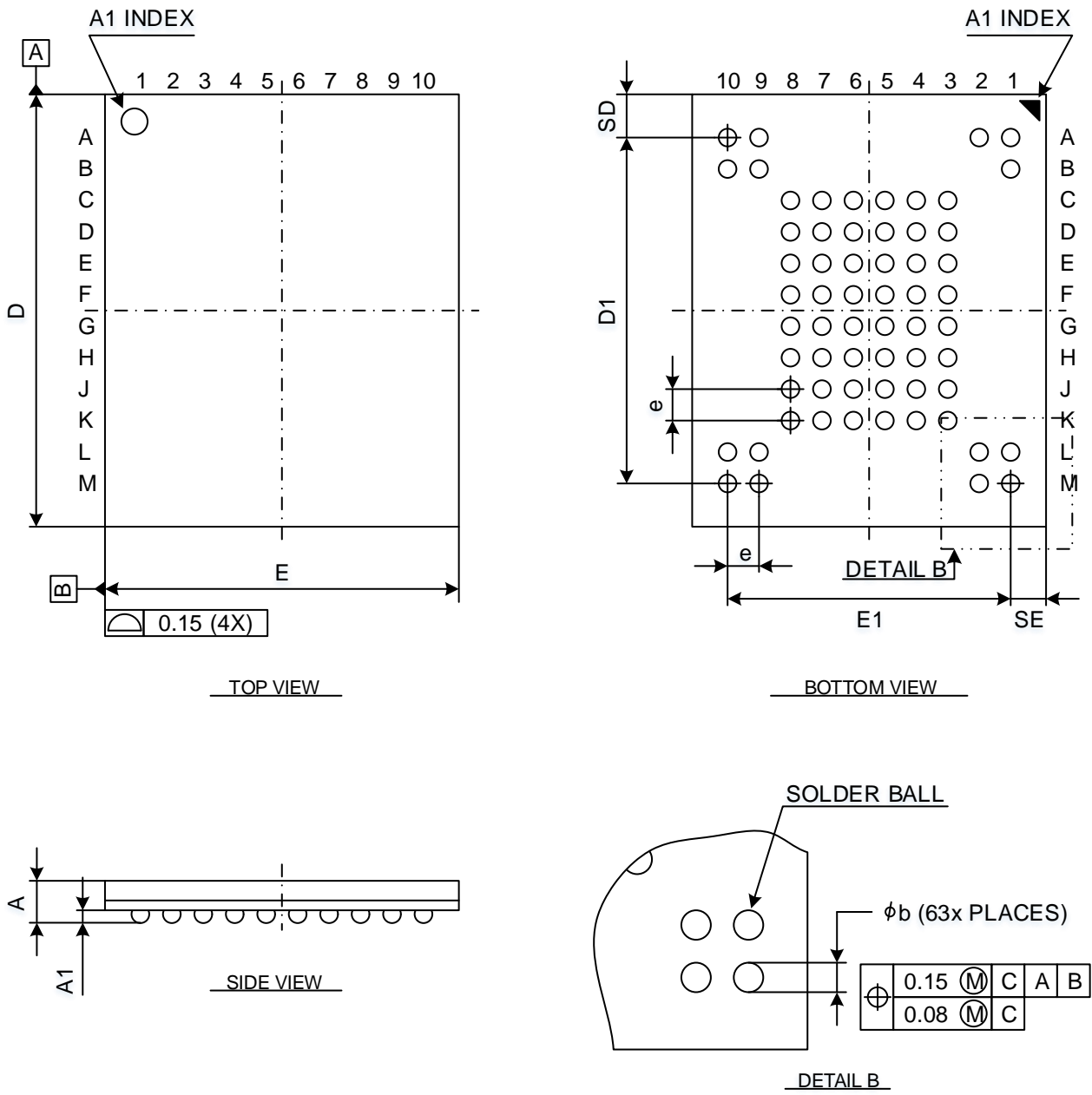
Figure 13-2: FBGA-63 figures
