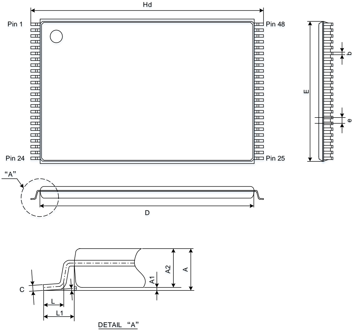
Figure 13-1: TSOPI-48 Figure
