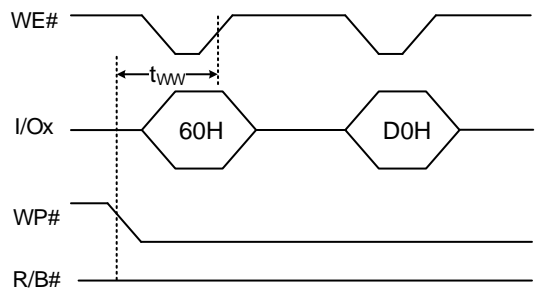
Figure 7-5_d: Write Protect Enable with erase figures
