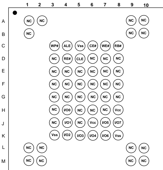
Figure 3-2_a: 63-FBGA Contact, x8 device
