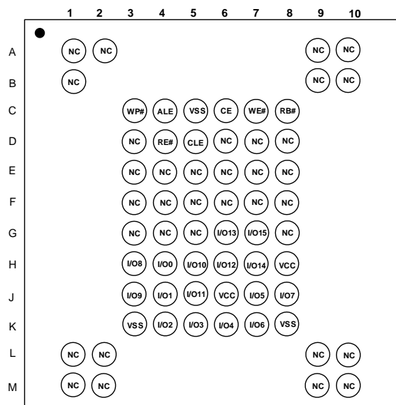
Figure 3-2_b: 63-FBGA Contact, x16 device
