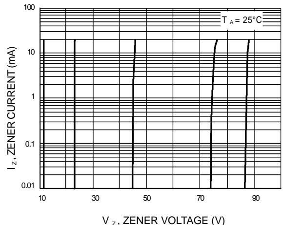
V_z , ZENER VOLTAGE (V) Figure 8. Zener Voltage versus Zener Current (12 V to 91 V)
