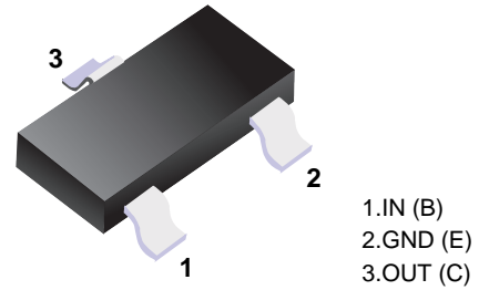
■ Simplified outline(SOT-23)
